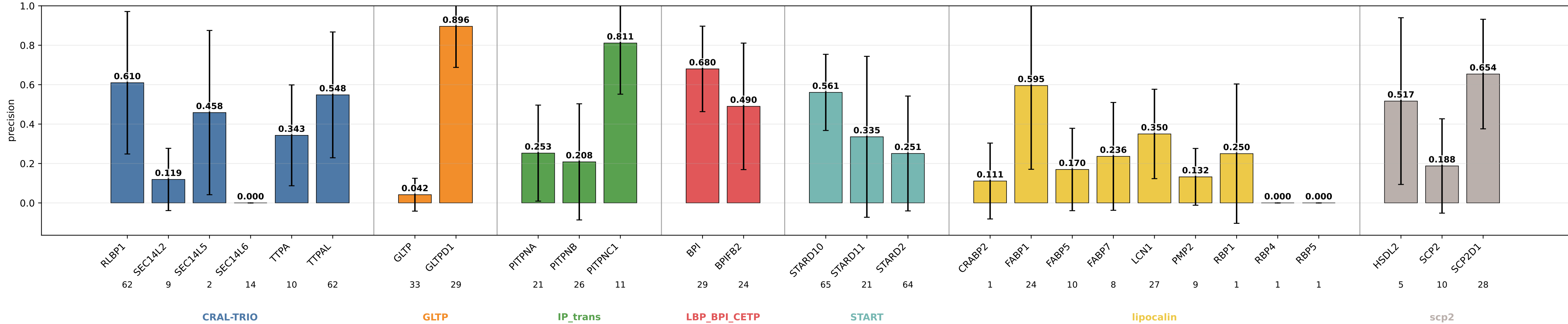
geometric_edge_attention_protgeom_family_neutral_normalized_bilinear_fusion_bilinear_norm_edge_orient_rbf6 precision by subgroup geometric_edge_attention_protgeom_family_neutral_normalized_bilinear_fusion_bilinear_norm_edge_orient_rbf6 | class weights | lr=0.0001 | weight_decay=0.01 | final_m=4 | final_dropout=0.1 | hiddim=8 | heads=8 | batch=16 | ep=120 | seeds=0,1,2,3,4
