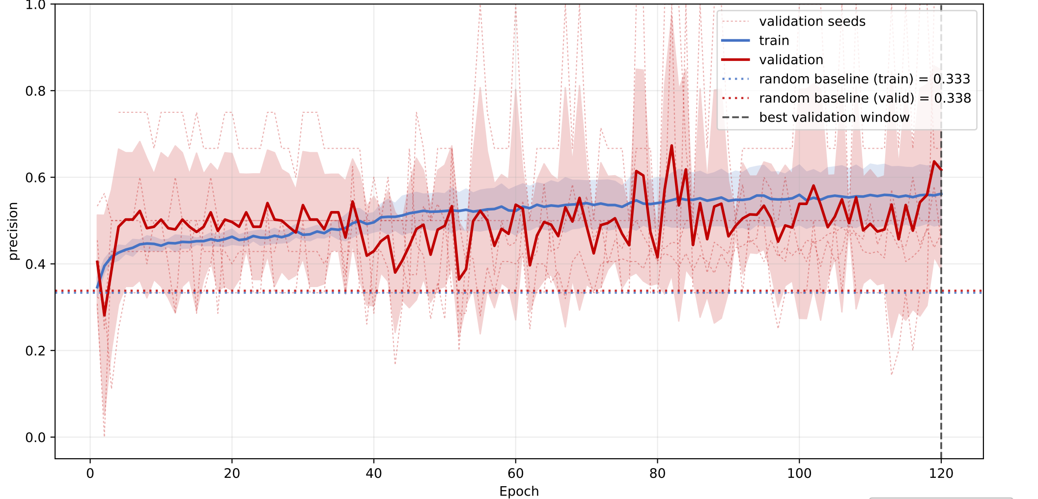
LBP_BPI_CETP: mean precision learning curve across seeds
