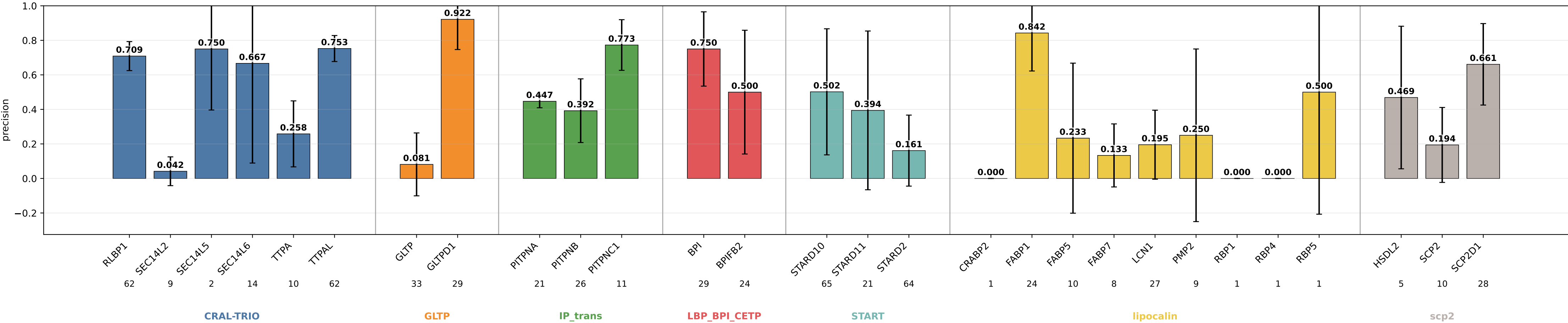
geometric_edge_attention_protgeom_family_neutral_normalized_bilinear_fusion_bilinear_norm_edge_rbf6 precision by subgroup geometric_edge_attention_protgeom_family_neutral_normalized_bilinear_fusion_bilinear_norm_edge_rbf6 | class weights | lr=0.0001 | weight_decay=0.01 | final_m=4 | final_dropout=0.1 | hiddim=8 | heads=8 | batch=16 | ep=120 | seeds=0,1,2,3,4
