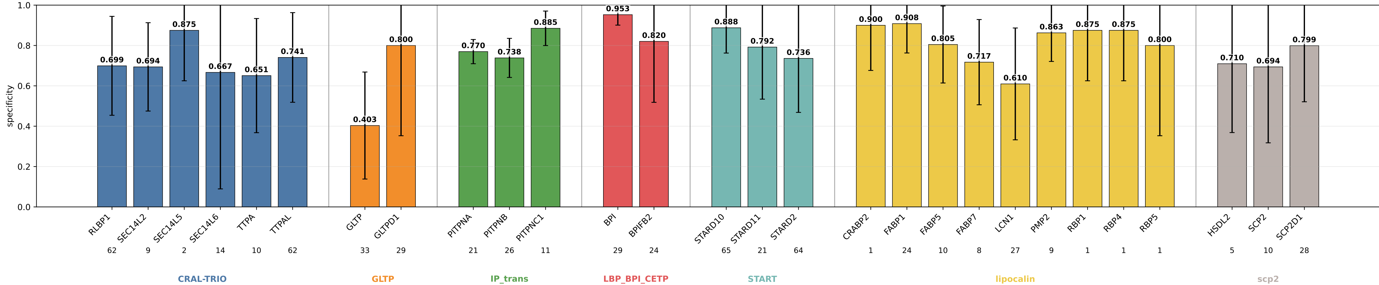
geometric_edge_attention_protgeom_family_neutral_normalized_bilinear_fusion_bilinear_norm_edge_rbf6 specificity by subgroup geometric_edge_attention_protgeom_family_neutral_normalized_bilinear_fusion_bilinear_norm_edge_rbf6 | class weights | lr=0.0001 | weight_decay=0.01 | final_m=4 | final_dropout=0.1 | hiddim=8 | heads=8 | batch=16 | ep=120 | seeds=0,1,2,3,4
