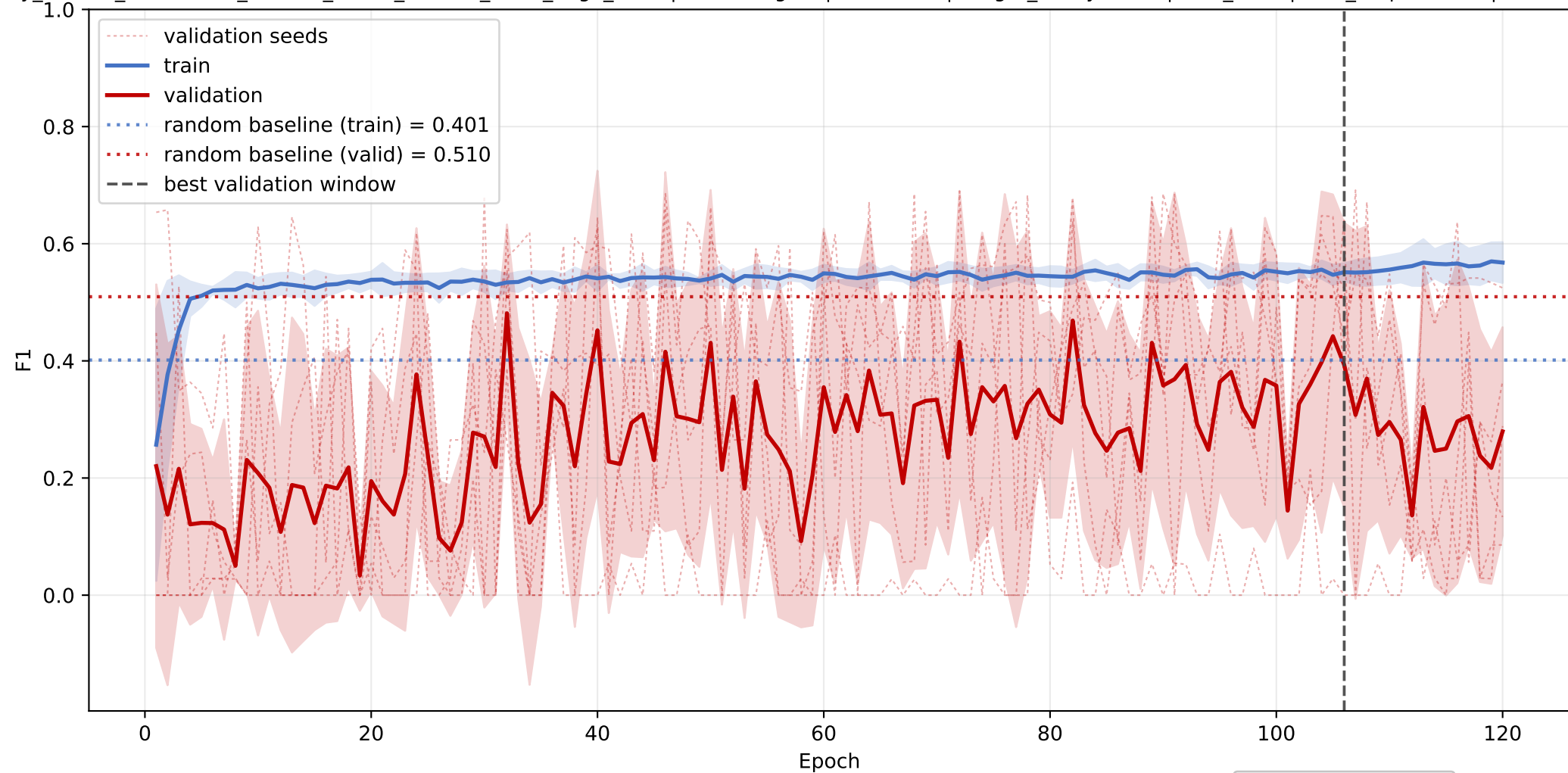
CRAL-TRIO: mean F1 learning curve across seeds
