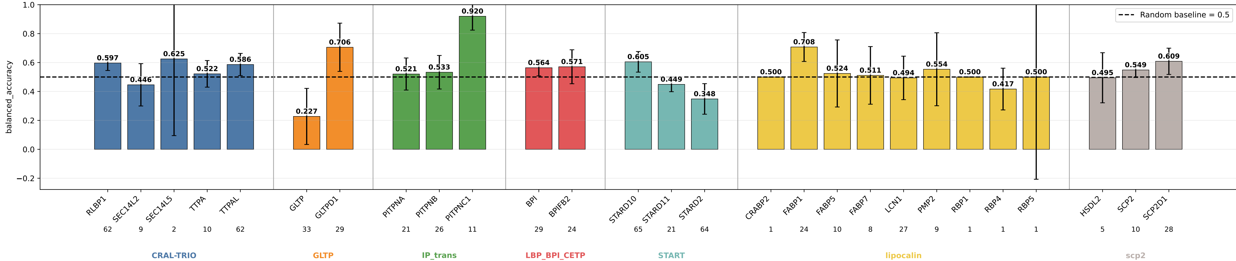
geometric_edge_mlp_protgeom_family_neutral_normalized_bilinear_fusion_bilinear_norm_edge_rbf6 balanced_accuracy by subgroup geometric_edge_mlp_protgeom_family_neutral_normalized_bilinear_fusion_bilinear_norm_edge_rbf6 | class weights | lr=0.0001 | weight_decay=0.01 | final_m=4 | final_dropout=0.1 | hiddim=8 | heads=8 | batch=16 | ep=120 | seeds=0,1,2,3,4
