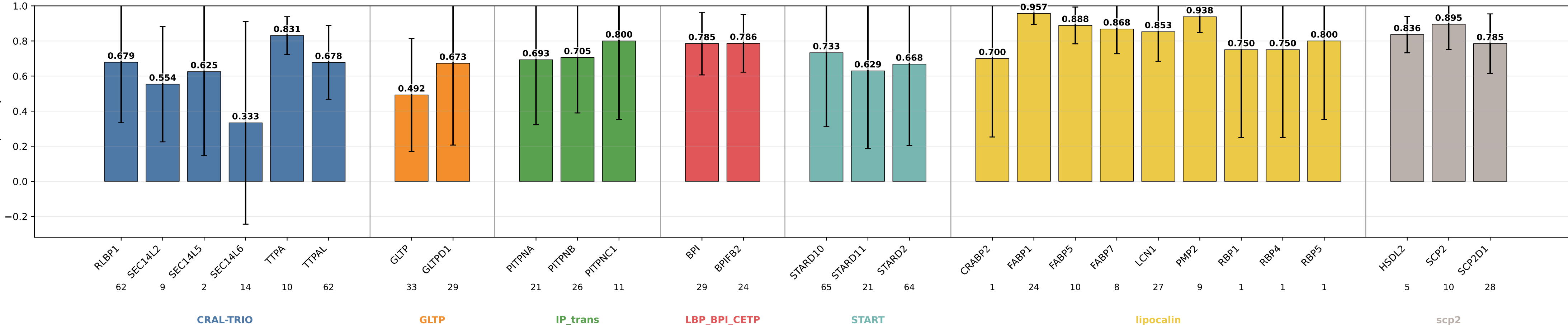
geometric_edge_mlp_protgeom_family_neutral_normalized_bilinear_fusion_bilinear_norm_node_bilinear specificity by subgroup geometric_edge_mlp_protgeom_family_neutral_normalized_bilinear_fusion_bilinear_norm_node_bilinear | class weights | lr=0.0001 | weight_decay=0.01 | final_m=4 | final_dropout=0.1 | hiddim=8 | heads=8 | batch=16 | ep=120 | seeds=0,1,2,3,4
