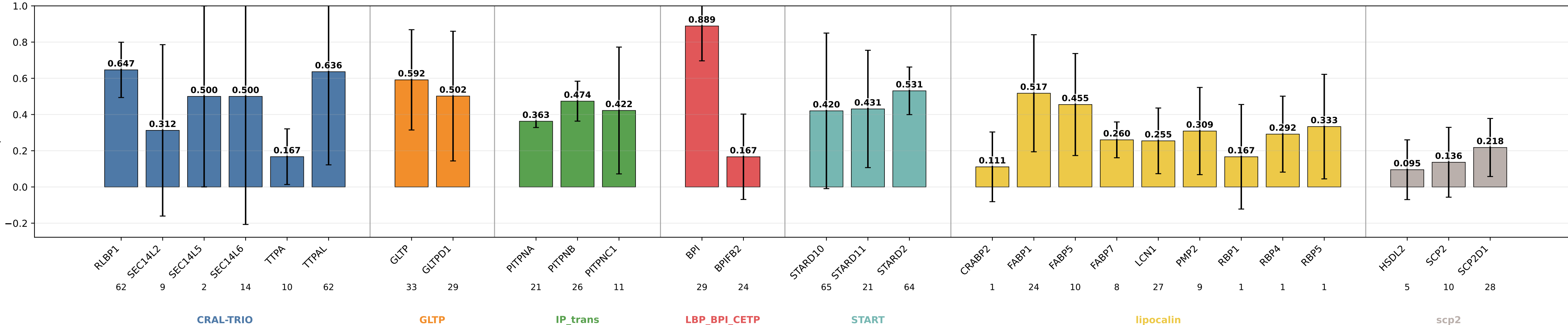
thematical_paths_geom_chem precision by subgroup thematical_paths_geom_chem | class weights | lr=0.0001 | weight_decay=0.01 | final_m=4 | final_dropout=0.1 | hiddim=8 | heads=8 | batch=16 | ep=120 | seeds=0,1,2,3,4
