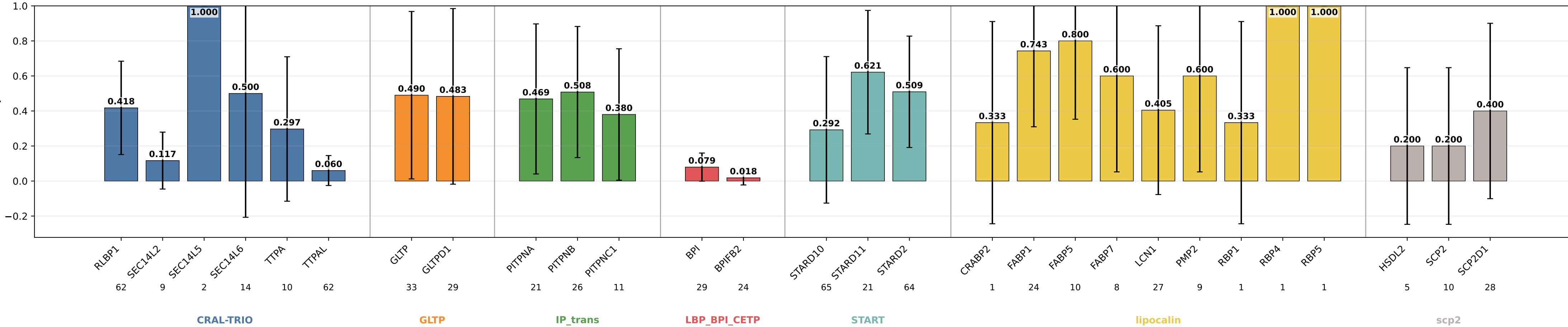
thematical_paths_geom_chem sensitivity by subgroup thematical_paths_geom_chem | class weights | lr=0.0001 | weight_decay=0.01 | final_m=4 | final_dropout=0.1 | hiddim=8 | heads=8 | batch=16 | ep=120 | seeds=0,1,2,3,4
