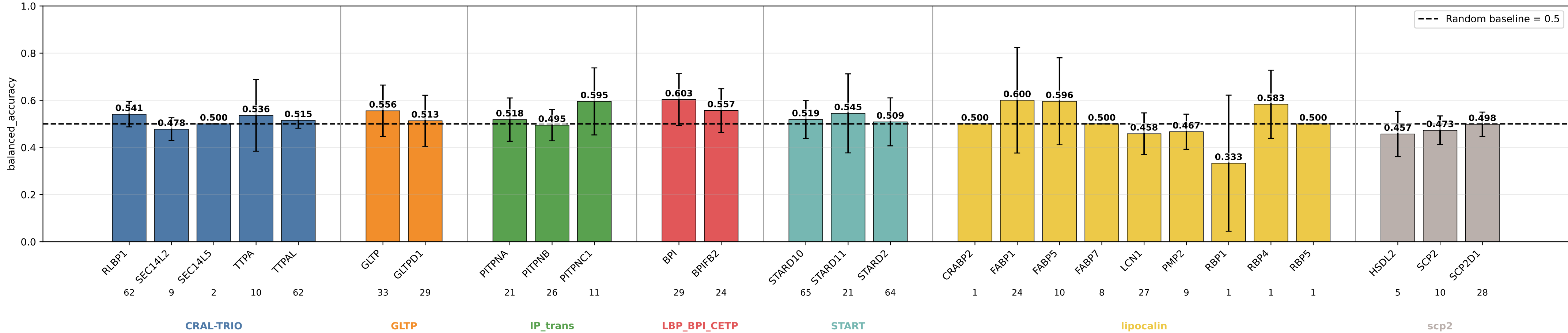
thematical_paths_geom_chem_bn_scale balanced_accuracy by subgroup thematical_paths_geom_chem_bn_scale | class weights | lr=0.0001 | weight_decay=0.01 | final_m=4 | final_dropout=0.1 | hiddim=8 | heads=8 | batch=16 | ep=120 | seeds=0,1,2,3,4
