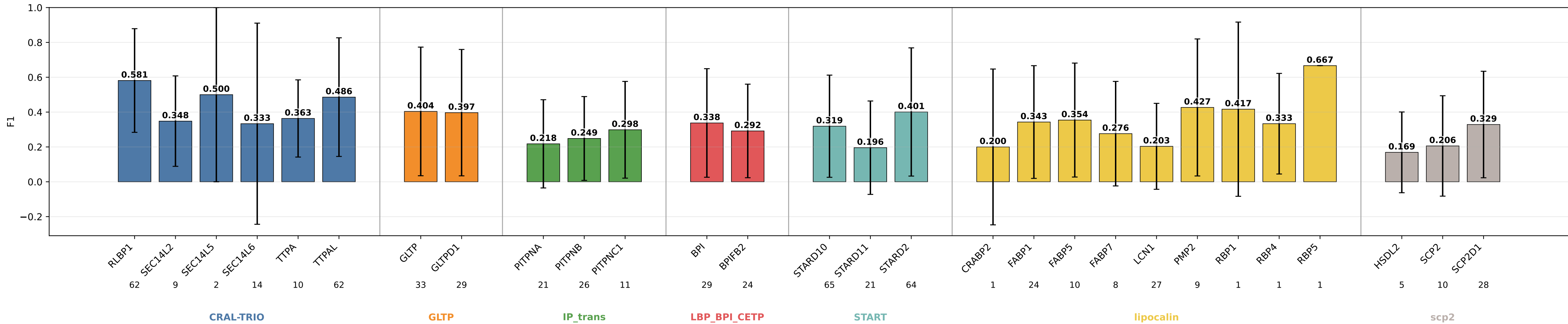
thematical_paths_geom_chem_interaction_lr F1 by subgroup thematical_paths_geom_chem_interaction_lr | class weights | lr=0.0001 | weight_decay=0.01 | final_m=4 | final_dropout=0.1 | hiddim=8 | heads=8 | batch=16 | ep=120 | seeds=0,1,2,3,4
