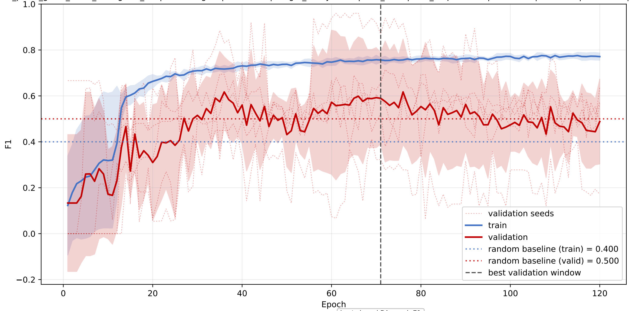
GLTP: mean F1 learning curve across seeds
