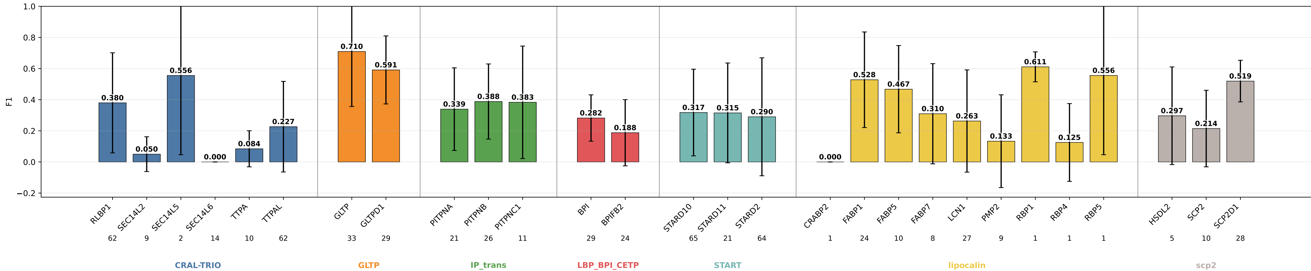
thematical_paths_geom_chem_orthogonal_init F1 by subgroup thematical_paths_geom_chem_orthogonal_init | class weights | lr=0.0001 | weight_decay=0.01 | final_m=4 | final_dropout=0.1 | hiddim=8 | heads=8 | batch=16 | ep=120 | seeds=0,1,2,3,4
