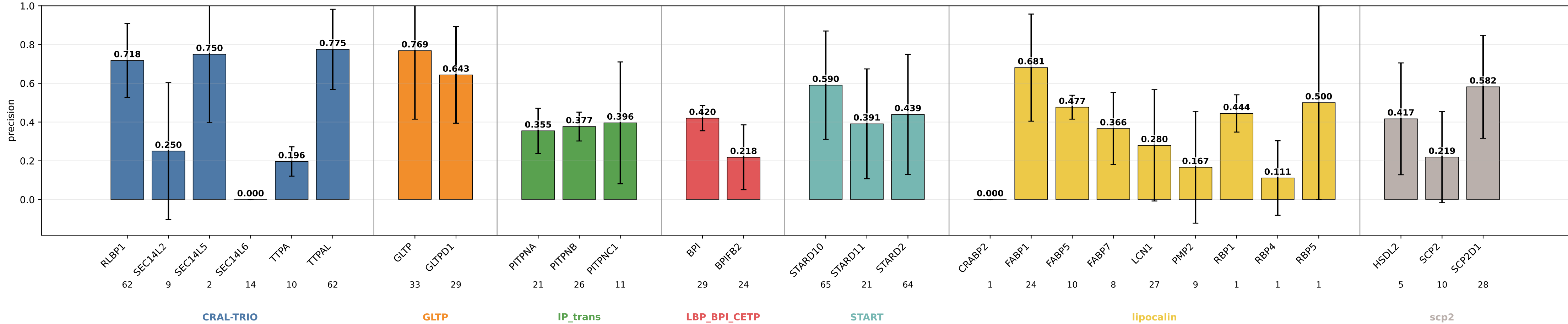
thematical_paths_geom_chem_orthogonal_init precision by subgroup thematical_paths_geom_chem_orthogonal_init | class weights | lr=0.0001 | weight_decay=0.01 | final_m=4 | final_dropout=0.1 | hiddim=8 | heads=8 | batch=16 | ep=120 | seeds=0,1,2,3,4
