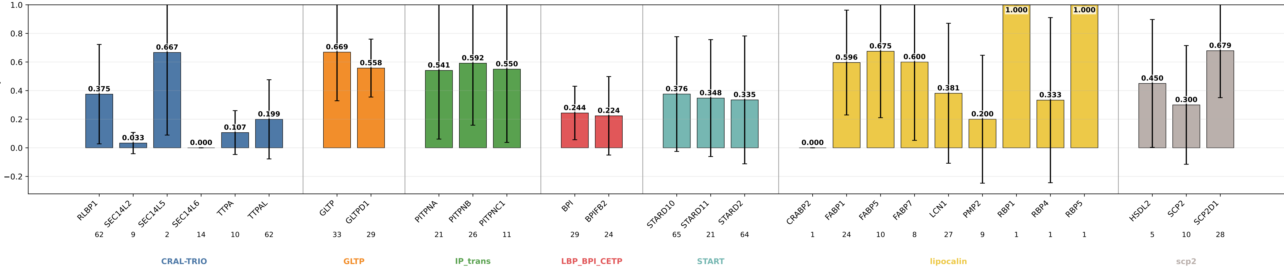
thematical_paths_geom_chem_orthogonal_init sensitivity by subgroup thematical_paths_geom_chem_orthogonal_init | class weights | lr=0.0001 | weight_decay=0.01 | final_m=4 | final_dropout=0.1 | hiddim=8 | heads=8 | batch=16 | ep=120 | seeds=0,1,2,3,4
