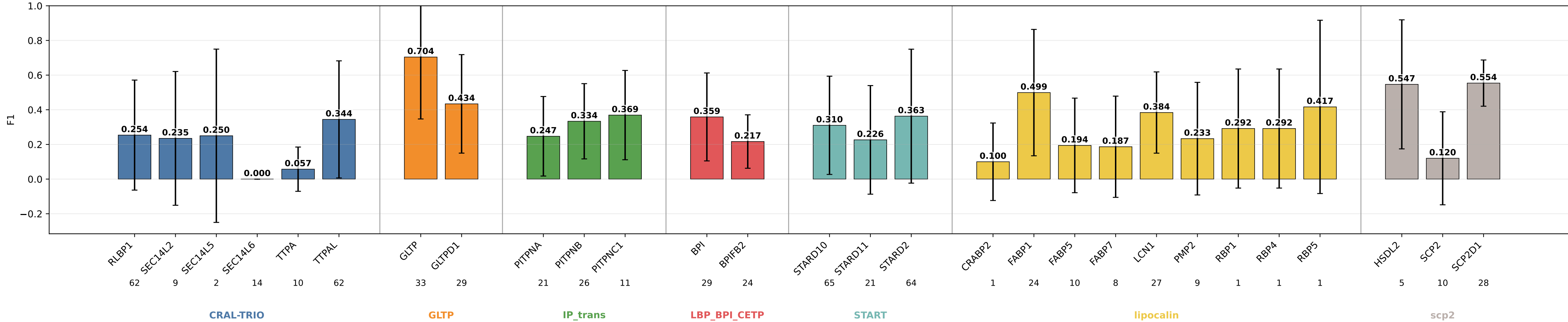
thematical_paths_geom_chem_orthogonal_init_batch64 F1 by subgroup thematical_paths_geom_chem_orthogonal_init_batch64 | class weights | lr=0.0001 | weight_decay=0.01 | final_m=4 | final_dropout=0.1 | hiddim=8 | heads=8 | batch=64 | ep=120 | seeds=0,1,2,3,4
