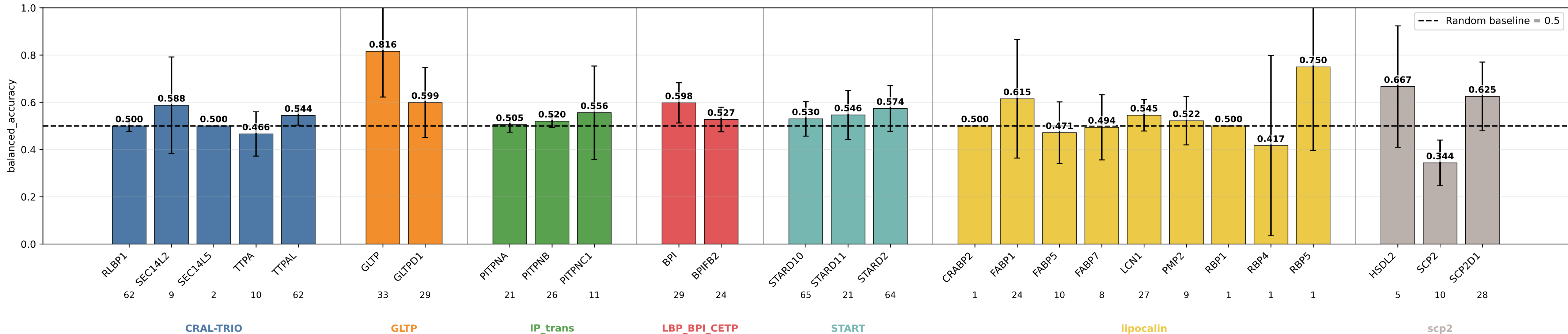
thematical_paths_geom_chem_orthogonal_init_batch64 balanced_accuracy by subgroup thematical_paths_geom_chem_orthogonal_init_batch64 | class weights | lr=0.0001 | weight_decay=0.01 | final_m=4 | final_dropout=0.1 | hiddim=8 | heads=8 | batch=64 | ep=120 | seeds=0,1,2,3,4
