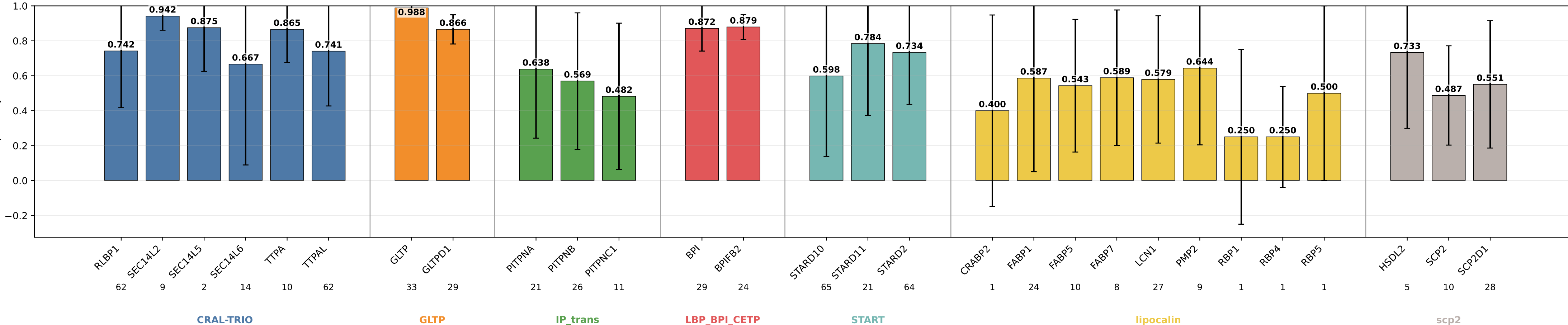
thematical_paths_geom_chem_orthogonal_init_batch64 specificity by subgroup thematical_paths_geom_chem_orthogonal_init_batch64 | class weights | lr=0.0001 | weight_decay=0.01 | final_m=4 | final_dropout=0.1 | hiddim=8 | heads=8 | batch=64 | ep=120 | seeds=0,1,2,3,4
