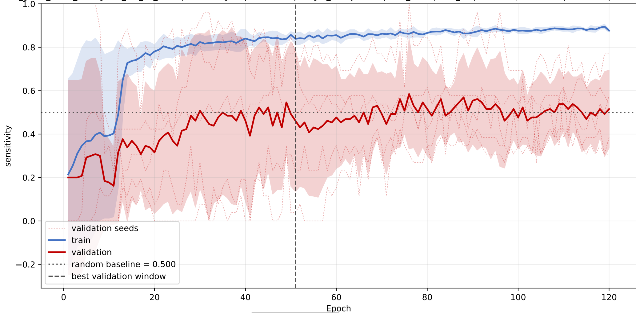
GLTP: mean sensitivity learning curve across seeds
