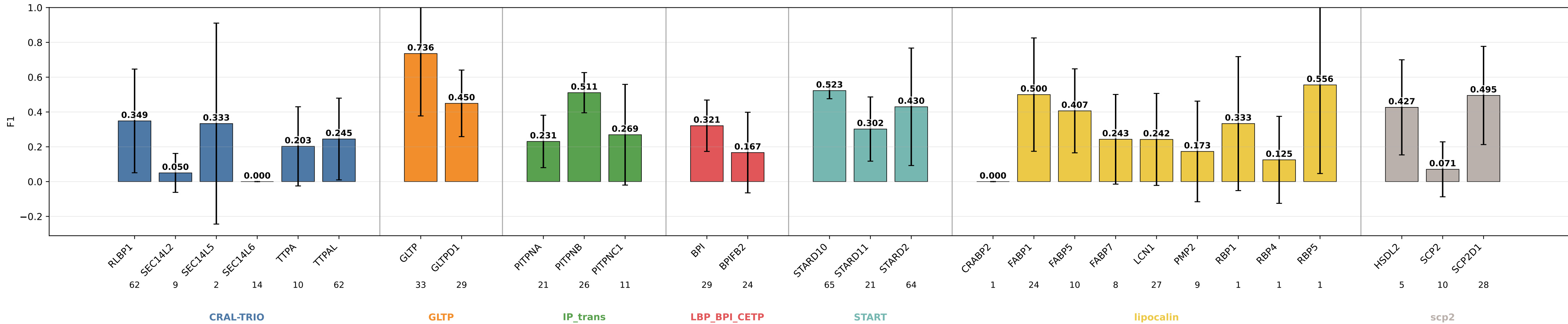
thematical_paths_geom_chem_orthogonal_init_bn_scale F1 by subgroup thematical_paths_geom_chem_orthogonal_init_bn_scale | class weights | lr=0.0001 | weight_decay=0.01 | final_m=4 | final_dropout=0.1 | hiddim=8 | heads=8 | batch=16 | ep=120 | seeds=0,1,2,3,4
