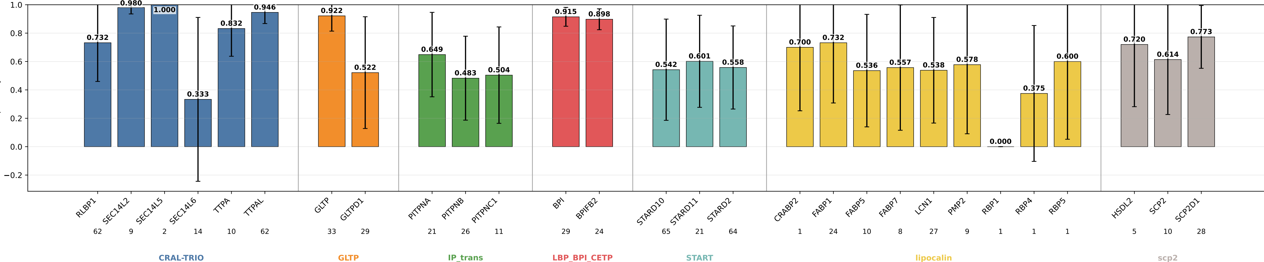
thematical_paths_geom_chem_orthogonal_init_bn_scale specificity by subgroup thematical_paths_geom_chem_orthogonal_init_bn_scale | class weights | lr=0.0001 | weight_decay=0.01 | final_m=4 | final_dropout=0.1 | hiddim=8 | heads=8 | batch=16 | ep=120 | seeds=0,1,2,3,4
