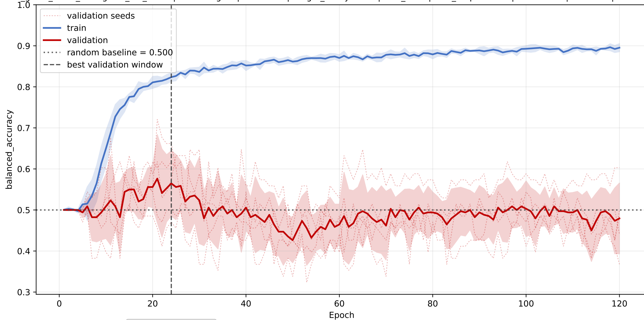
scp2: mean balanced_accuracy learning curve across seeds
