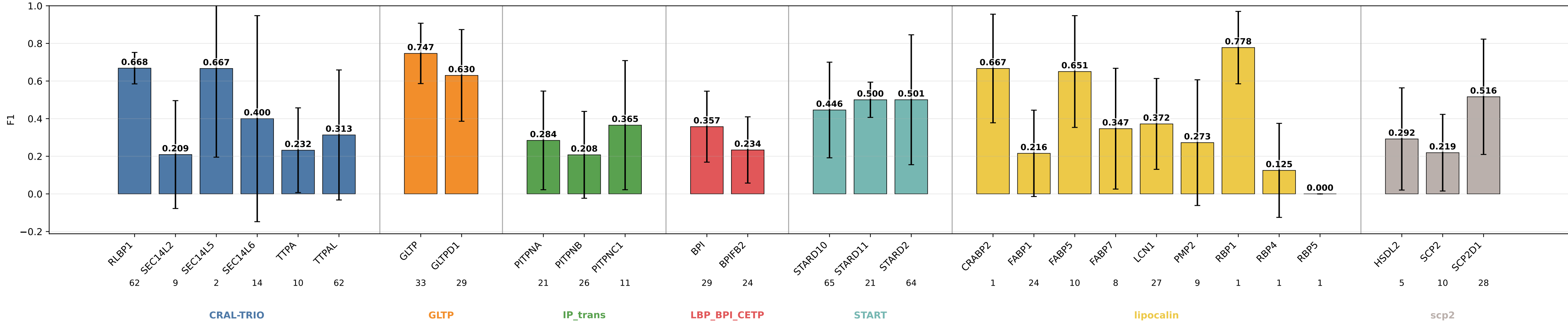
thematical_paths_geom_chem_ortweight05 F1 by subgroup thematical_paths_geom_chem_ortweight05 | class weights | lr=0.0001 | weight_decay=0.01 | final_m=4 | final_dropout=0.1 | hiddim=8 | heads=8 | batch=16 | ep=120 | seeds=0,1,2,3,4
