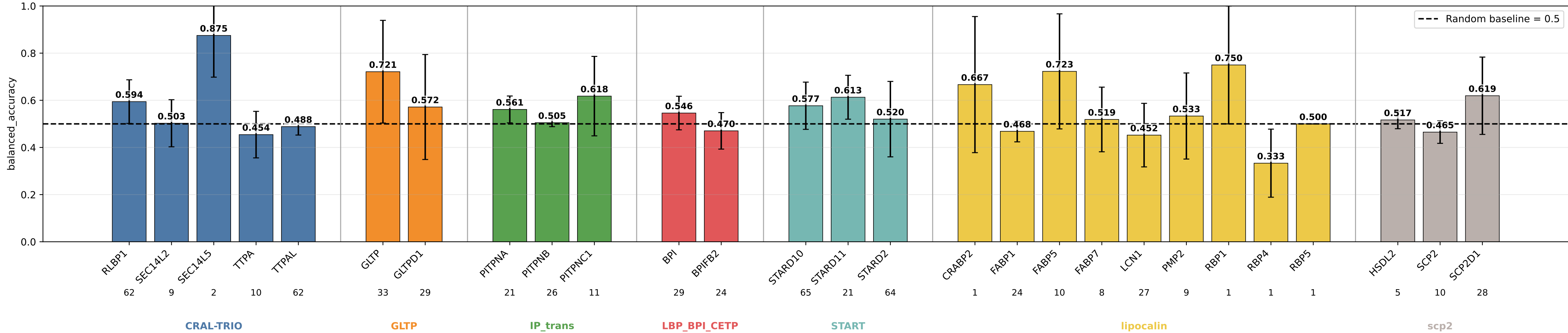
thematical_paths_geom_chem_ortweight05 balanced_accuracy by subgroup thematical_paths_geom_chem_ortweight05 | class weights | lr=0.0001 | weight_decay=0.01 | final_m=4 | final_dropout=0.1 | hiddim=8 | heads=8 | batch=16 | ep=120 | seeds=0,1,2,3,4
