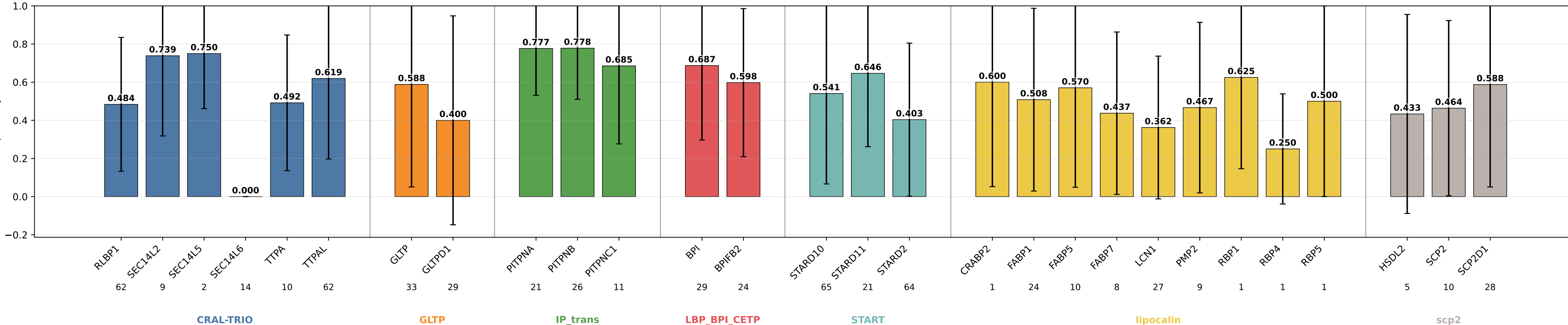
thematical_paths_geom_chem_ortweight05 specificity by subgroup thematical_paths_geom_chem_ortweight05 | class weights | lr=0.0001 | weight_decay=0.01 | final_m=4 | final_dropout=0.1 | hiddim=8 | heads=8 | batch=16 | ep=120 | seeds=0,1,2,3,4
