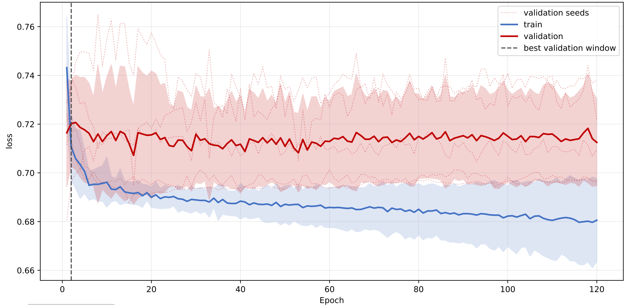
OSBP: mean loss learning curve across seeds
