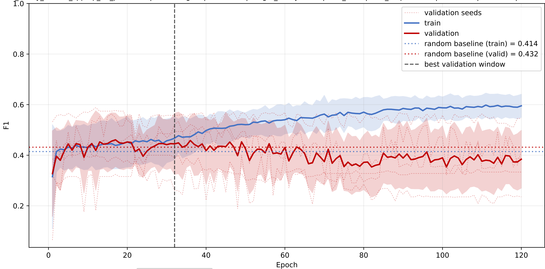
phosphorus_free: mean F1 learning curve across seeds
