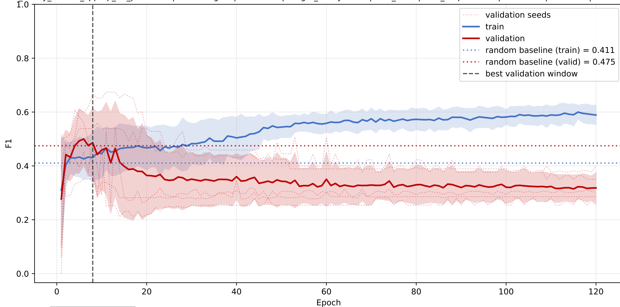
sphingolipids: mean F1 learning curve across seeds
