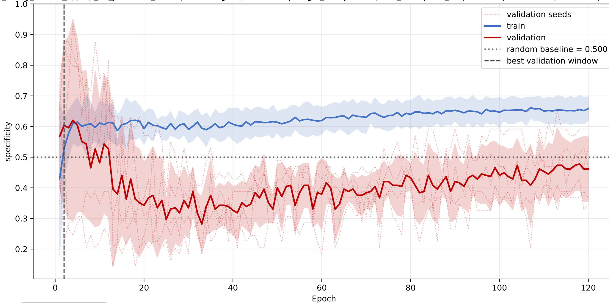
phosphorus_free: mean specificity learning curve across seeds
