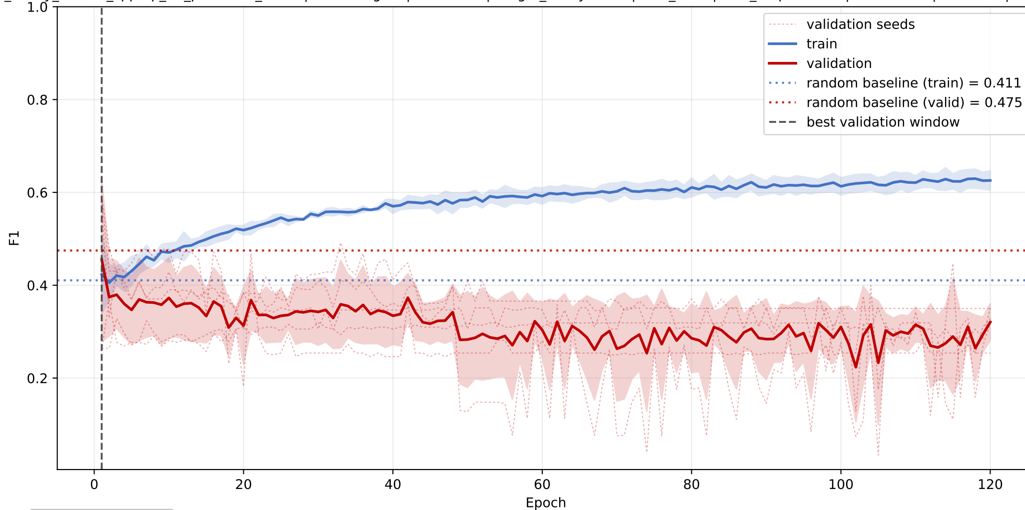
sphingolipids: mean F1 learning curve across seeds
