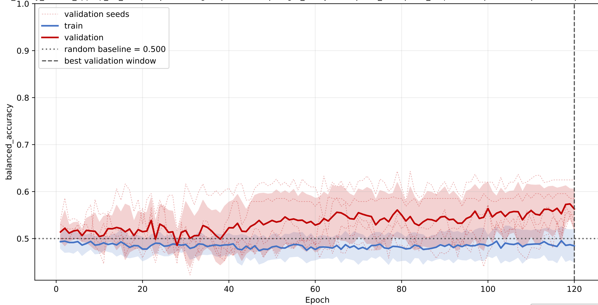
phosphorus_free: mean balanced_accuracy learning curve across seeds
