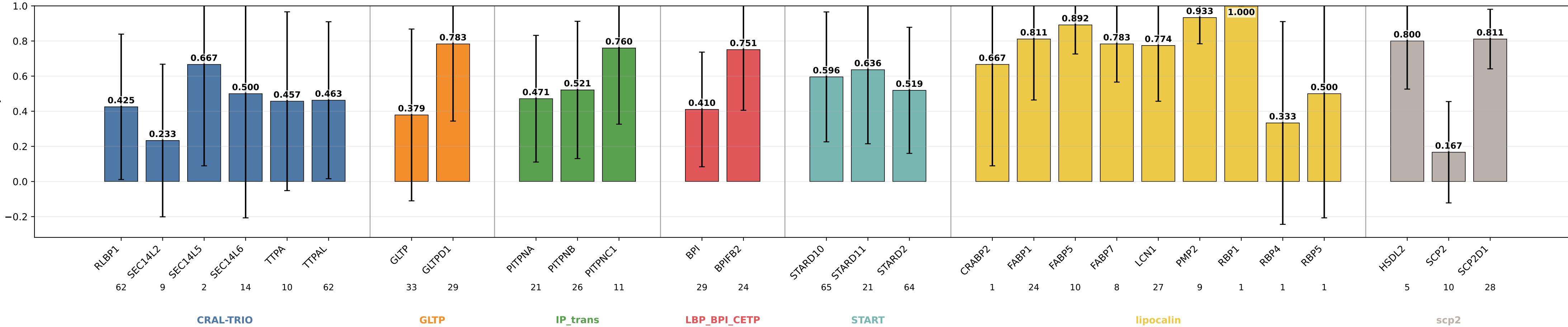
descriptors_head_family_neutral_lipprop_pair sensitivity by subgroup descriptors_head_family_neutral_lipprop_pair | class weights | lr=0.0001 | weight_decay=0.01 | final_m=4 | final_dropout=0.1 | hiddim=8 | heads=8 | batch=16 | ep=120 | seeds=0,1,2,3,4
