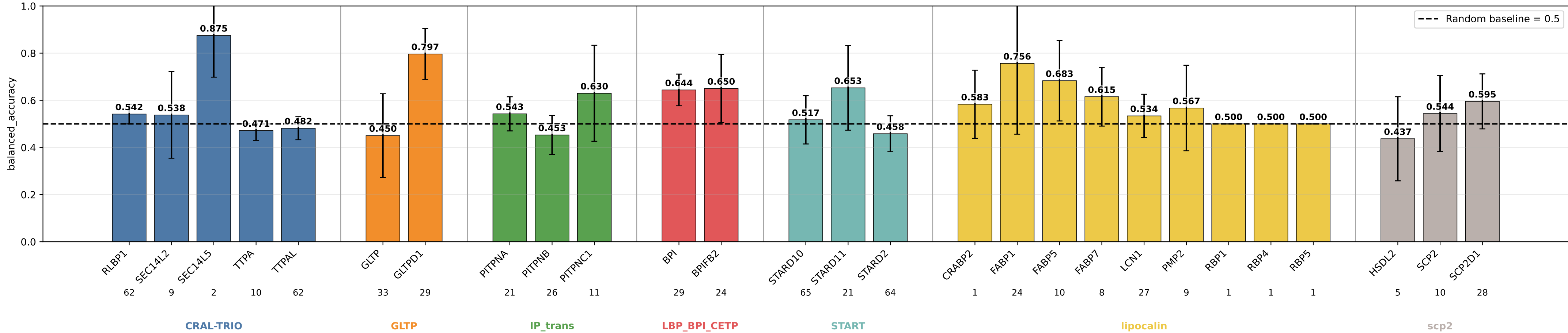
descriptors_pair_clean balanced_accuracy by subgroup descriptors_pair_clean | class weights | lr=0.0001 | weight_decay=0.01 | final_m=4 | final_dropout=0.1 | hiddim=8 | heads=8 | batch=16 | ep=120 | seeds=0,1,2,3,4
