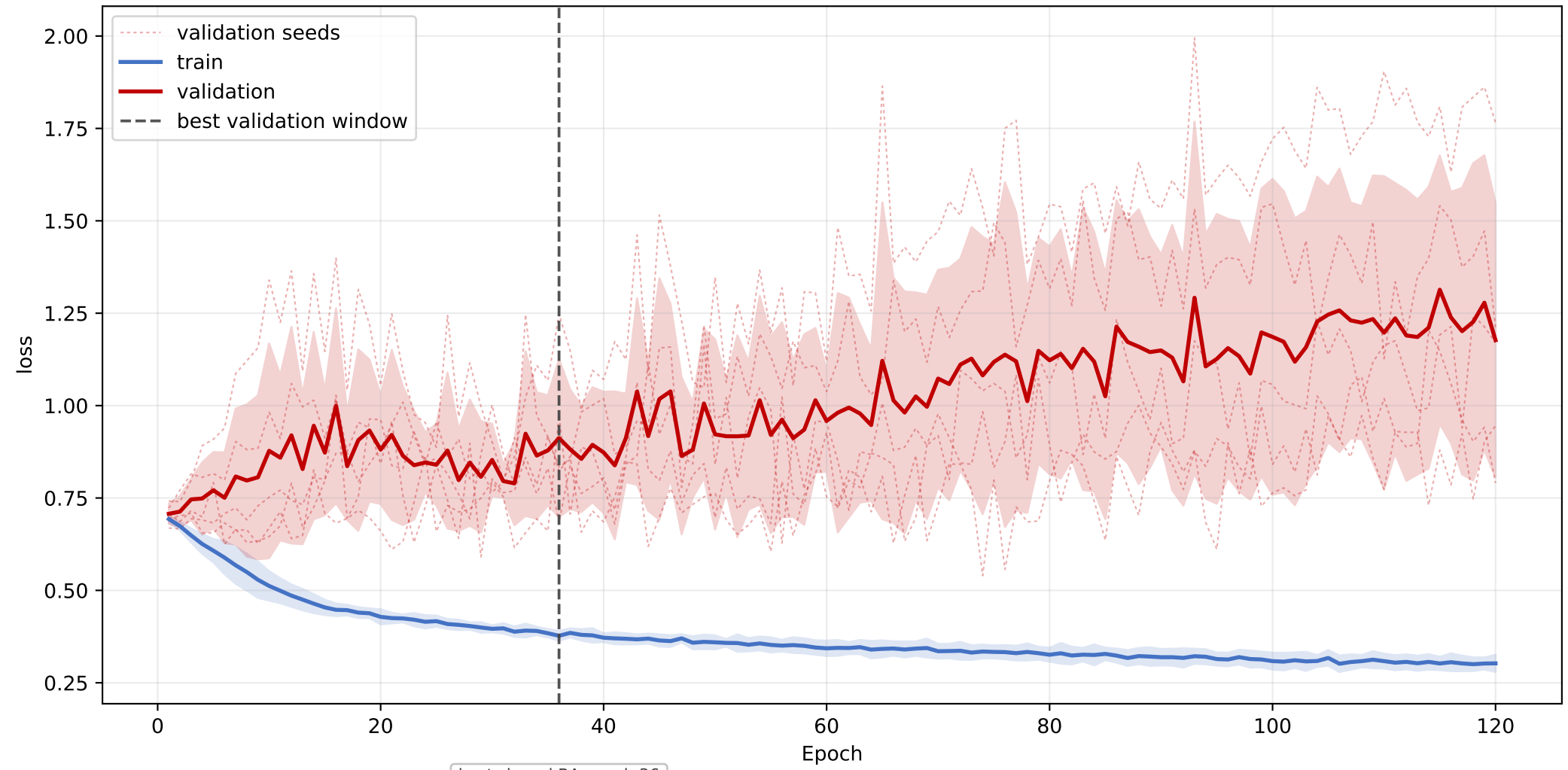
phosphorus_free: mean loss learning curve across seeds
