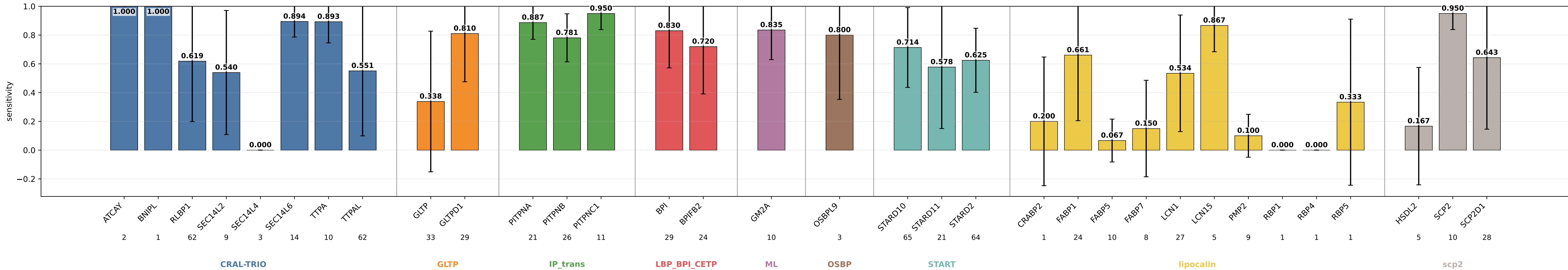
geometric_edge_mlp_protgeom_family_neutral_normalized_bilinear_fusion_bilinear_norm_lcs_esm3_balanced_lipid_classes_advprot_protfull sensitivity by subgroup geometric_edge_mlp_protgeom_family_neutral_normalized_bilinear_fusion_bilinear_norm_lcs_esm3_balanced_lipid_classes_advprot_protfull | class weights | lr=0.0001 | weight_decay=0.01 | final_m=4 | final_dropout=0.1 | hiddim=8 | heads=8 | batch=16 | ep=120 | seeds=0,1,2,3,4
