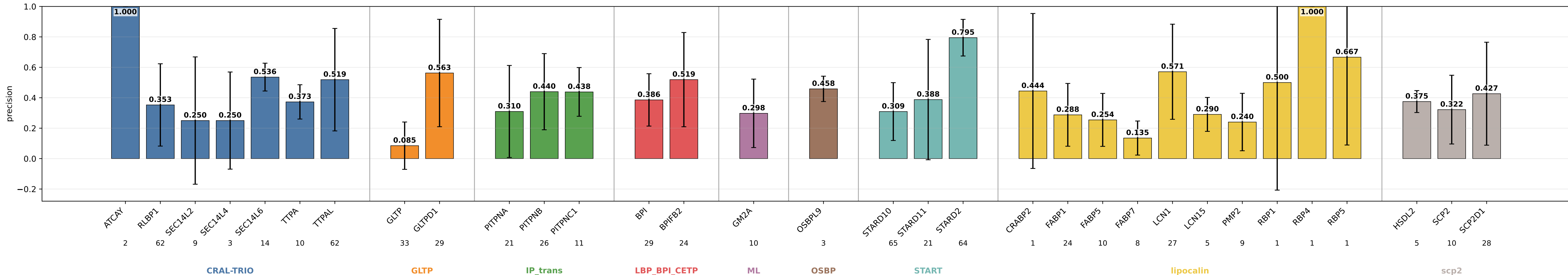
geometric_edge_mlp_protgeom_family_neutral_normalized_bilinear_fusion_bilinear_norm_lcs_protbind6_prothid32 precision by subgroup geometric_edge_mlp_protgeom_family_neutral_normalized_bilinear_fusion_bilinear_norm_lcs_protbind6_prothid32 | class weights | lr=0.0001 | weight_decay=0.01 | final_m=4 | final_dropout=0.1 | hiddim=8 | heads=8 | batch=16 | ep=120 | seeds=0,1,2,3,4
