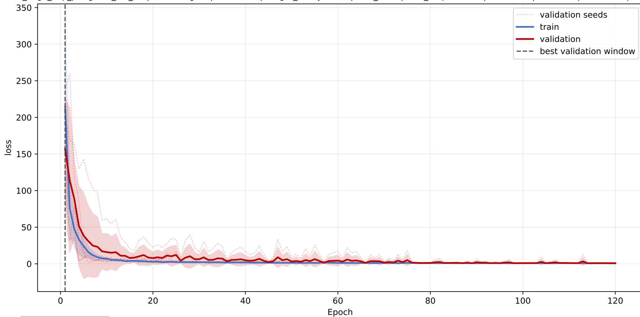
anionic: mean loss learning curve across seeds
