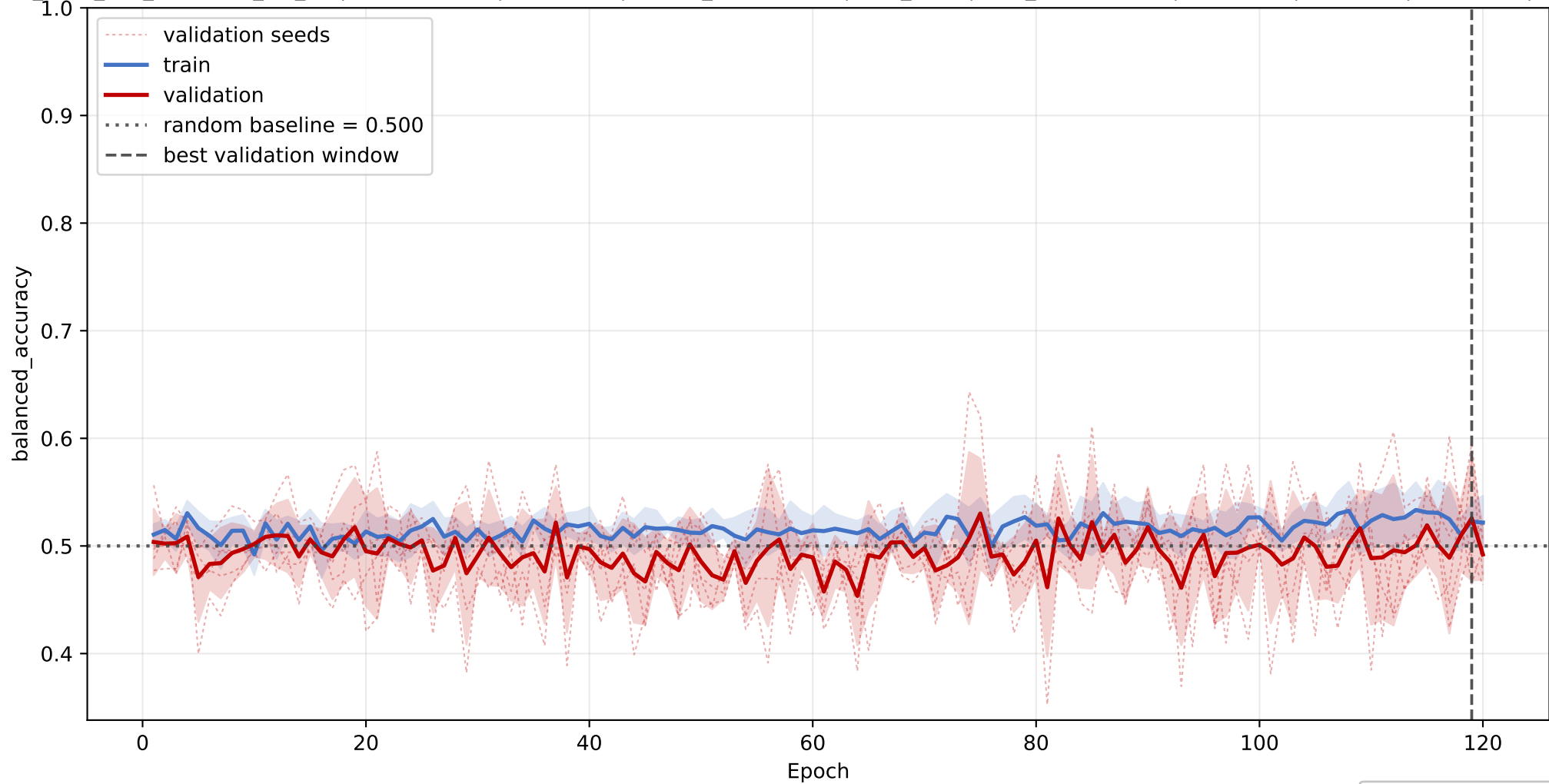
sphingolipids: mean balanced_accuracy learning curve across seeds
