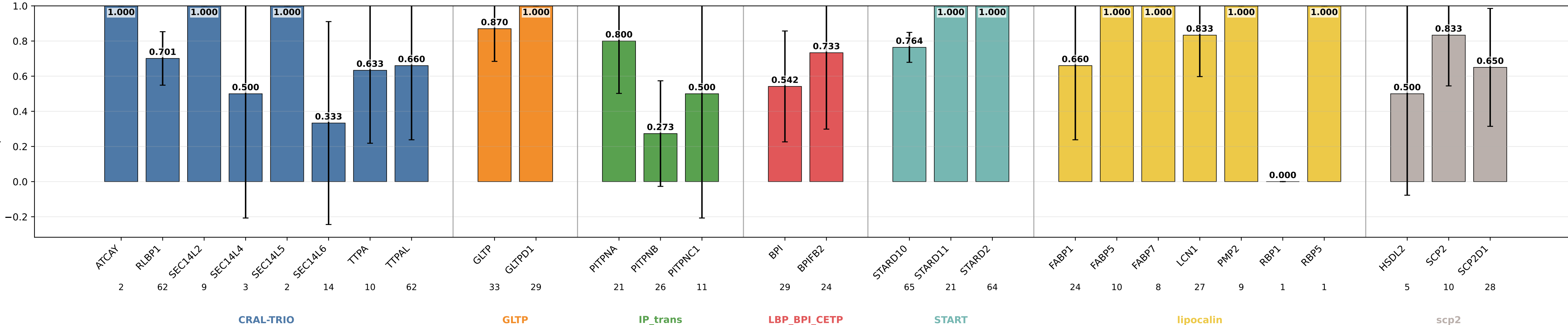
structural_pretrain_family_unfrozen_protunion14 precision by subgroup structural_pretrain_family_unfrozen_protunion14 | class weights | lr=0.0001 | weight_decay=0.001 | final_m=4 | final_dropout=0.1 | hiddim=64 | heads=8 | batch=16 | ep=120 | seeds=0,1,2,3,4
