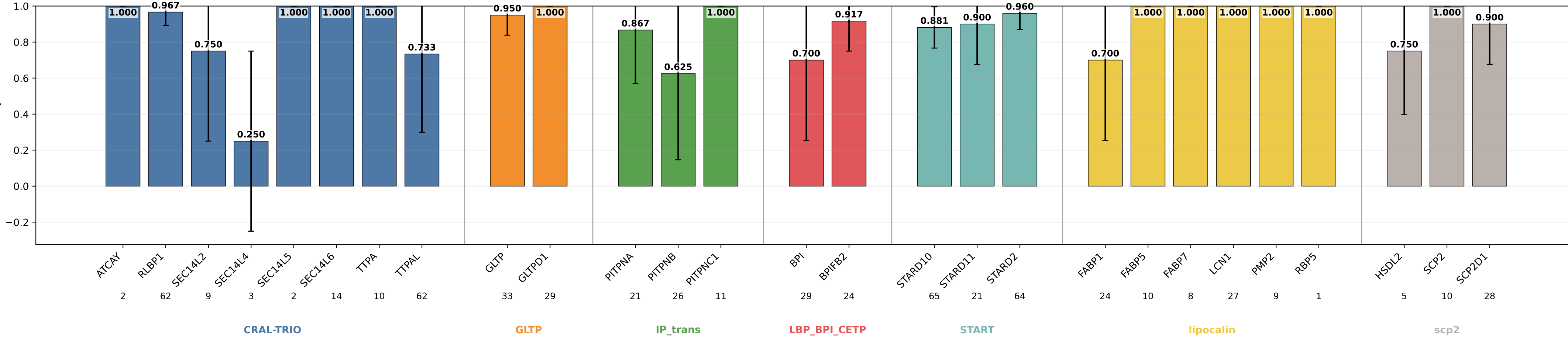
structural_pretrain_family_unfrozen_protunion14 sensitivity by subgroup structural_pretrain_family_unfrozen_protunion14 | class weights | lr=0.0001 | weight_decay=0.001 | final_m=4 | final_dropout=0.1 | hiddim=64 | heads=8 | batch=16 | ep=120 | seeds=0,1,2,3,4
