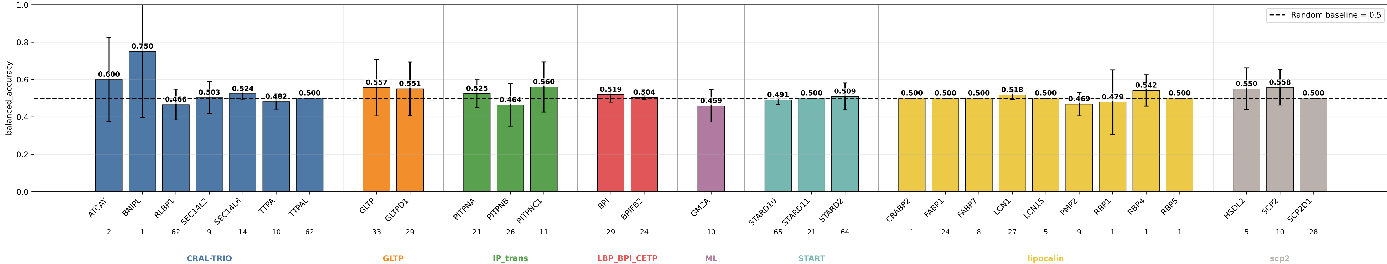
descriptors_head_family_neutral_lipprop_lcs_protbind6_rotneg balanced_accuracy by subgroup descriptors_head_family_neutral_lipprop_lcs_protbind6_rotneg | class weights | lr=0.0001 | weight_decay=0.01 | final_m=4 | final_dropout=0.1 | hiddim=8 | heads=8 | batch=16 | ep=120 | seeds=0,1,2,3,4
