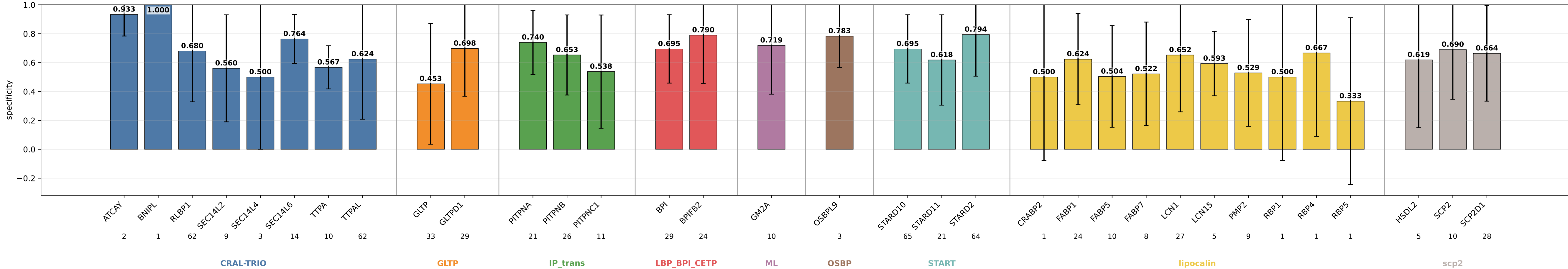
geometric_edge_mlp_protgeom_family_neutral_normalized_bilinear_fusion_bilinear_norm_lcs specificity by subgroup geometric_edge_mlp_protgeom_family_neutral_normalized_bilinear_fusion_bilinear_norm_lcs | class weights | lr=0.0001 | weight_decay=0.01 | final_m=4 | final_dropout=0.1 | hiddim=8 | heads=8 | batch=16 | ep=120 | seeds=0,1,2,3,4
