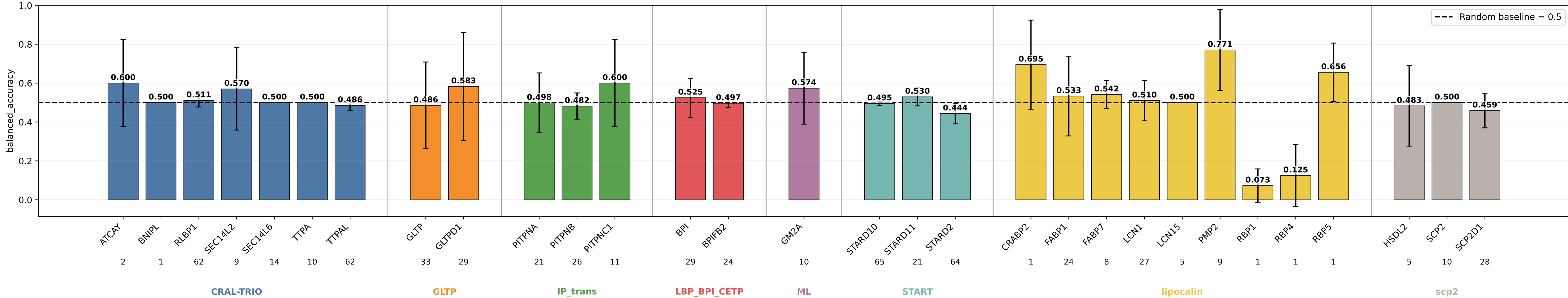
geometric_edge_mlp_protgeom_family_neutral_normalized_bilinear_fusion_bilinear_norm_lcs_esm3_balanced_lipid_classes balanced_accuracy by subgroup geometric_edge_mlp_protgeom_family_neutral_normalized_bilinear_fusion_bilinear_norm_lcs_esm3_balanced_lipid_classes | class weights | lr=0.0001 | weight_decay=0.01 | final_m=4 | final_dropout=0.1 | hiddim=8 | heads=8 | batch=16 | ep=120 | seeds=0,1,2,3,4
