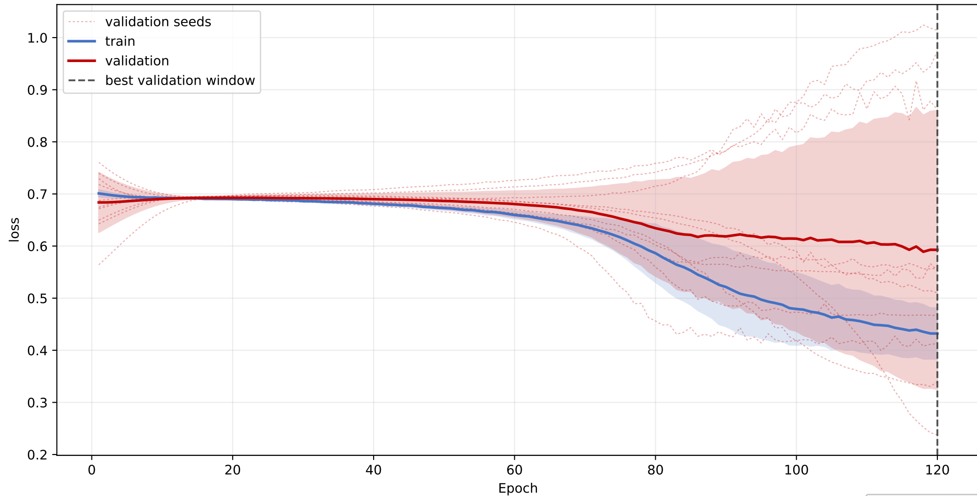
gltp: mean loss learning curve across seeds
