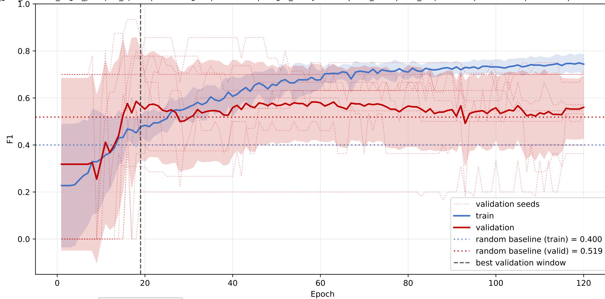
CerP+Hex2Cer+SHexCer_groups_gltf: mean F1 learning curve across seeds
