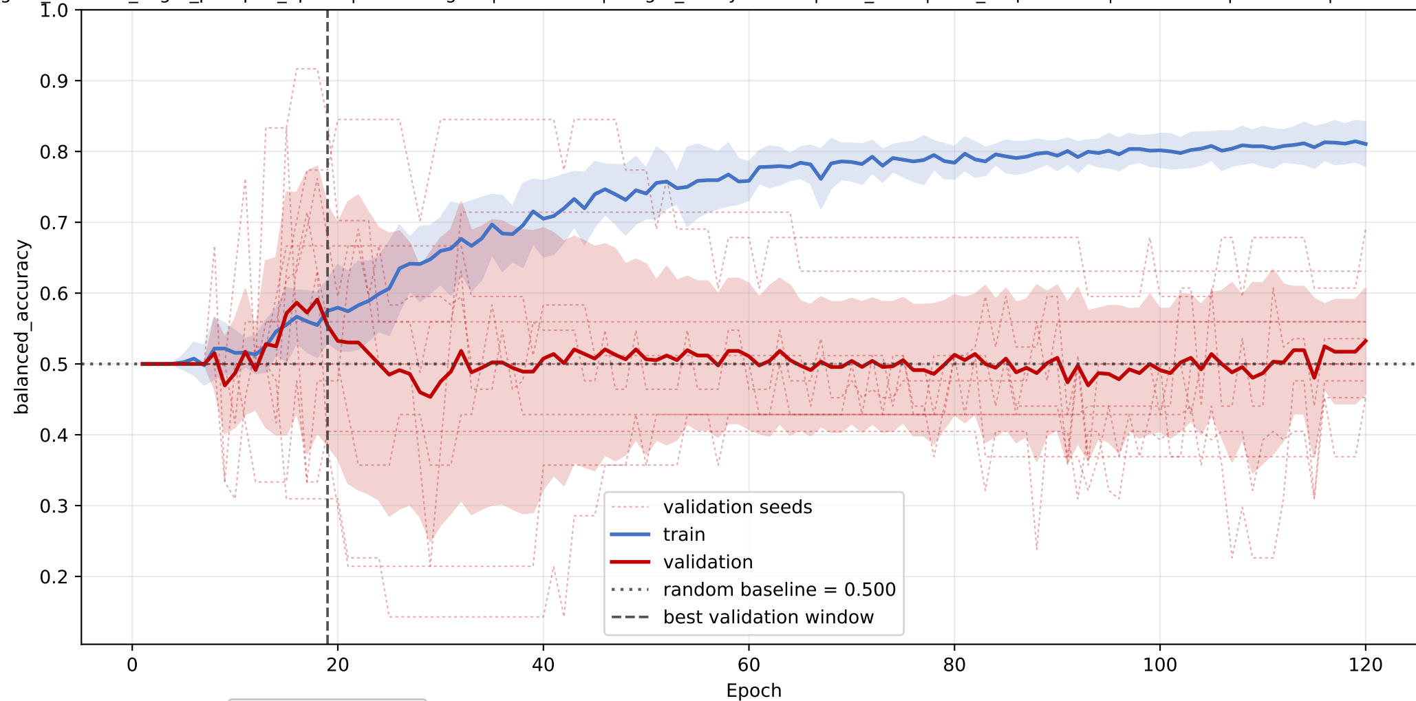
CerP+Hex2Cer+SHeCer_groups_glt: mean balanced_accuracy learning curve across seeds
