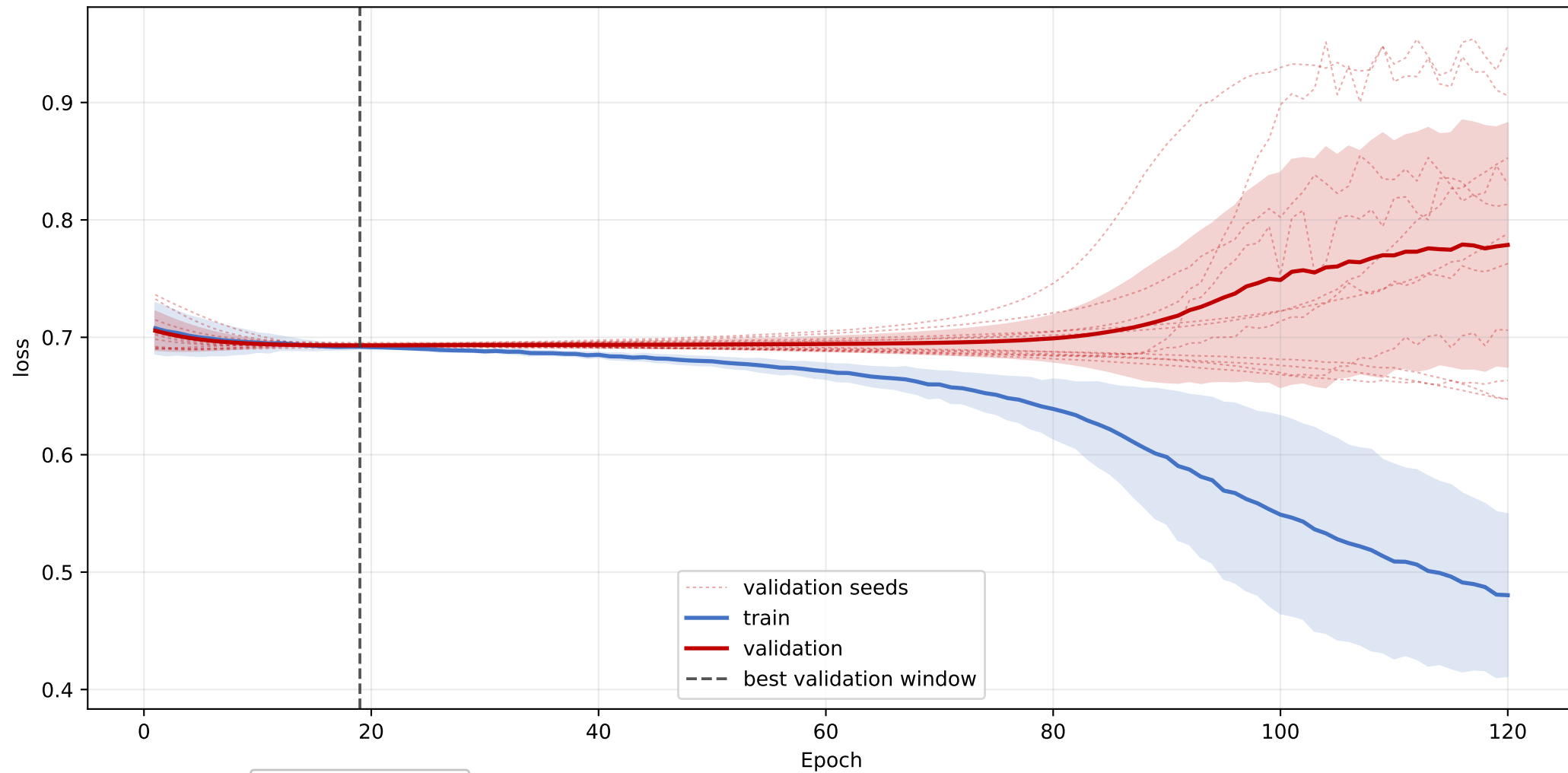
CerP+Hex2Cer+SHexCer_groups_gltip: mean loss learning curve across seeds
