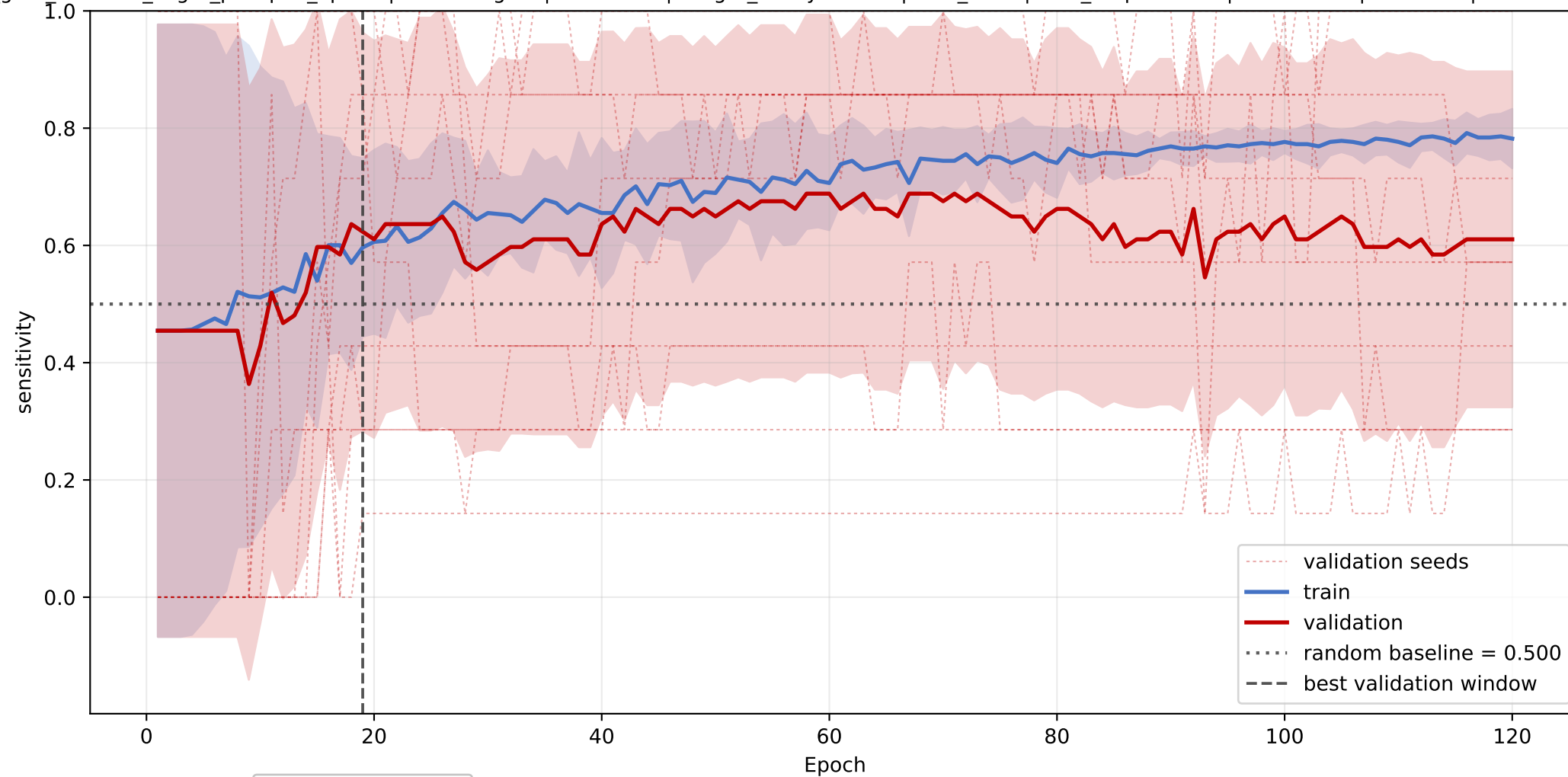
CerP+Hex2Cer+SHexCer_groups_gltf: mean sensitivity learning curve across seeds
