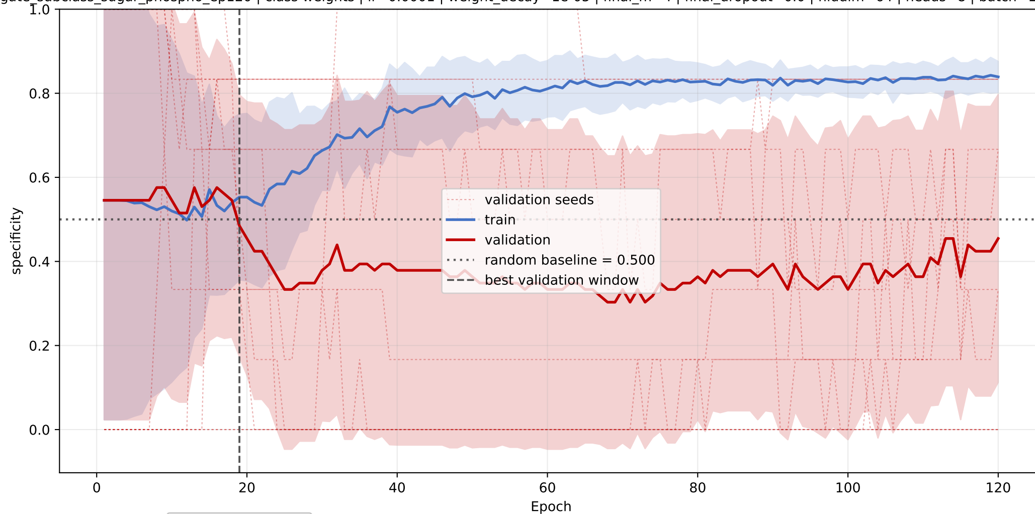
CerP+Hex2Cer+SHexCer_groups_gltf: mean specificity learning curve across seeds
