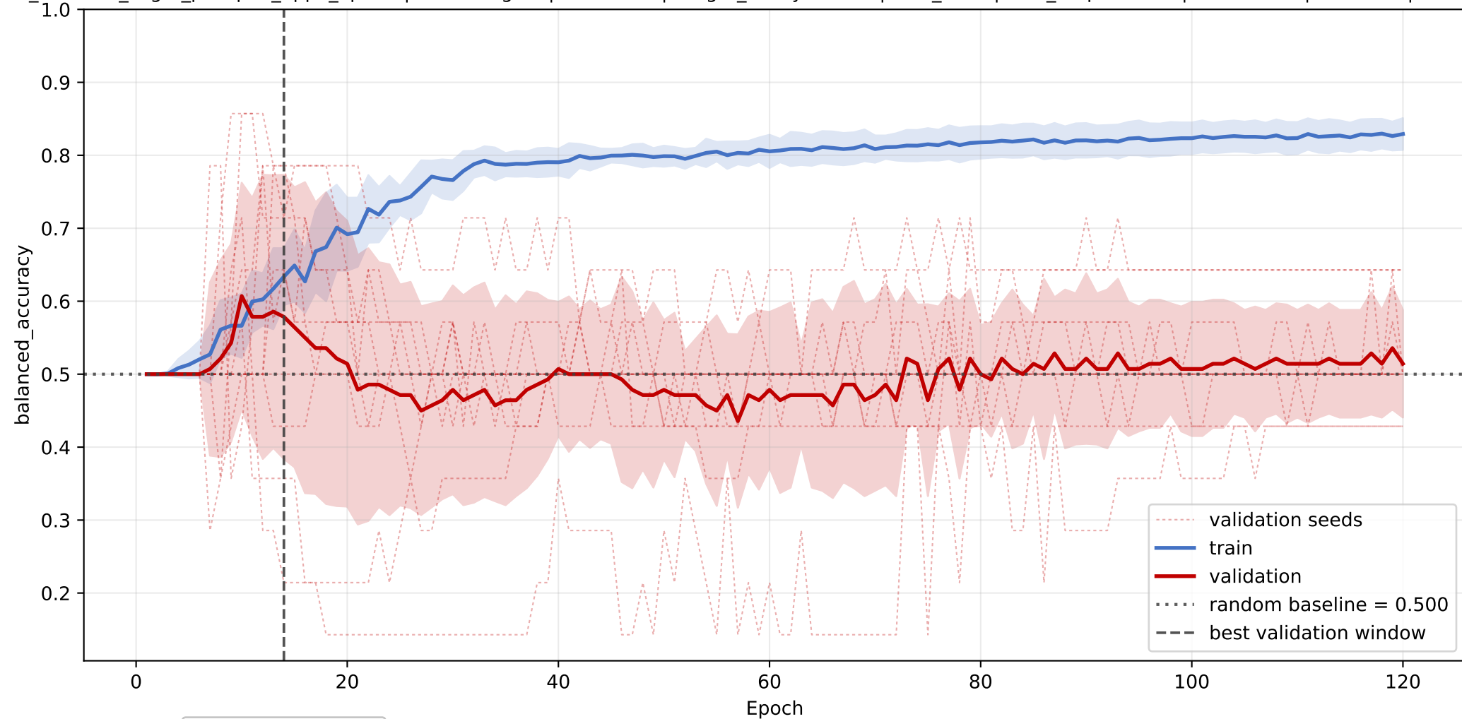
CerP+Hex2Cer+SHexCer_groups_glt: mean balanced_accuracy learning curve across seeds
